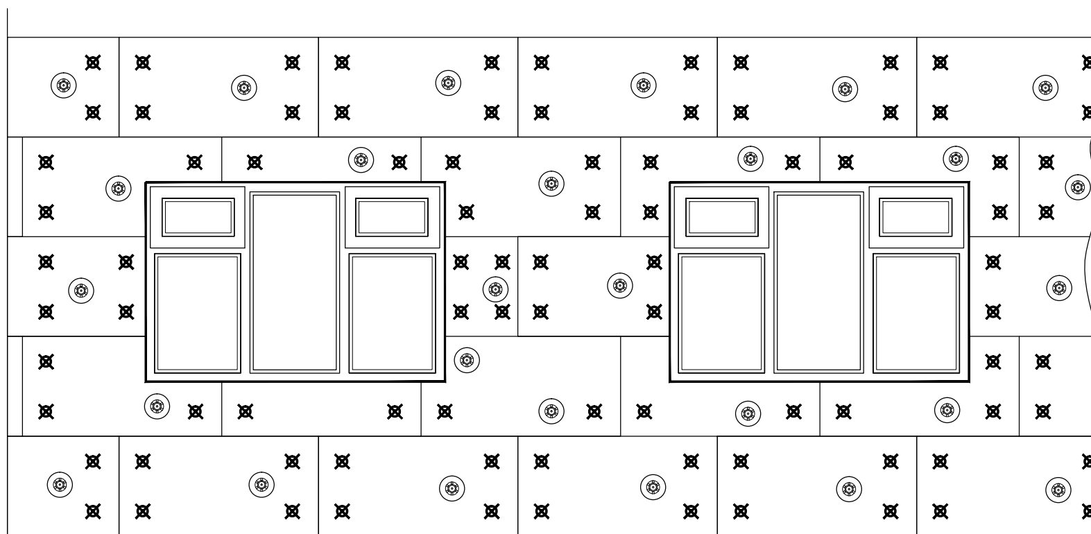
STAGE 2 - AFTER FIRST BASE COAT AND MESHING INSTALL ADDITIONAL FIXINGS AND FIRE FIXING
