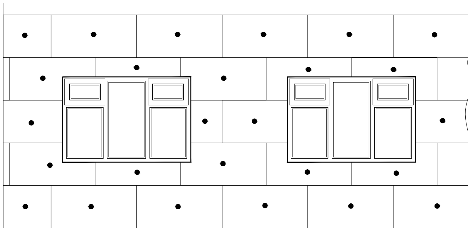
STAGE 1 - INSTALL INSULATION BOARD WITH A SINGLE FIXING
